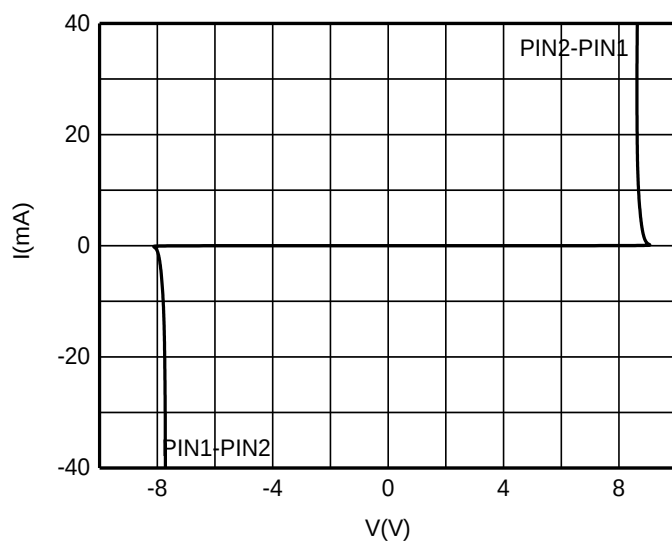
I-V Curve
